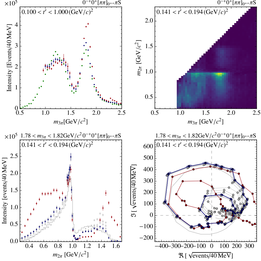
Figure 6.11.: Similar to fig. 6.7, now showing the 0^{-+}0^{+}[\pi\pi]_{0^{++}}\pi S wave. The red points show the direct results from the freed-isobar PWA without correcting for the zero mode. The blue points show the result after correction for the zero mode with the weighted average of the individual methods. The gray points in the bottom-row plots show the results of the individual methods. The picture in the upper left shows the incoherent sum over all four t' bins; the other three pictures only show results for a single t' bin.
