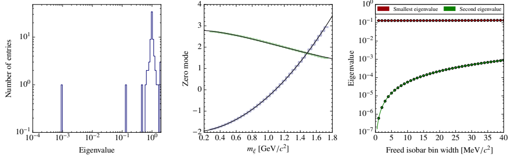
Figure 5.1.: Left: eigenvalue spectrum of the example model \pi(1800) \rightarrow [\pi\pi]_S \pi^- and [\pi\pi]_P \pi^- specified in section 5.2.5. Center: binned shapes of the zero mode for the S-wave in blue and P-wave in green. The corresponding black lines show the continuous shapes given in eq. (5.36) and eq. (5.37). Right: Dependence of the two smallest eigenvalues of the phase-space integral matrix on the freed-isobar bin width.
