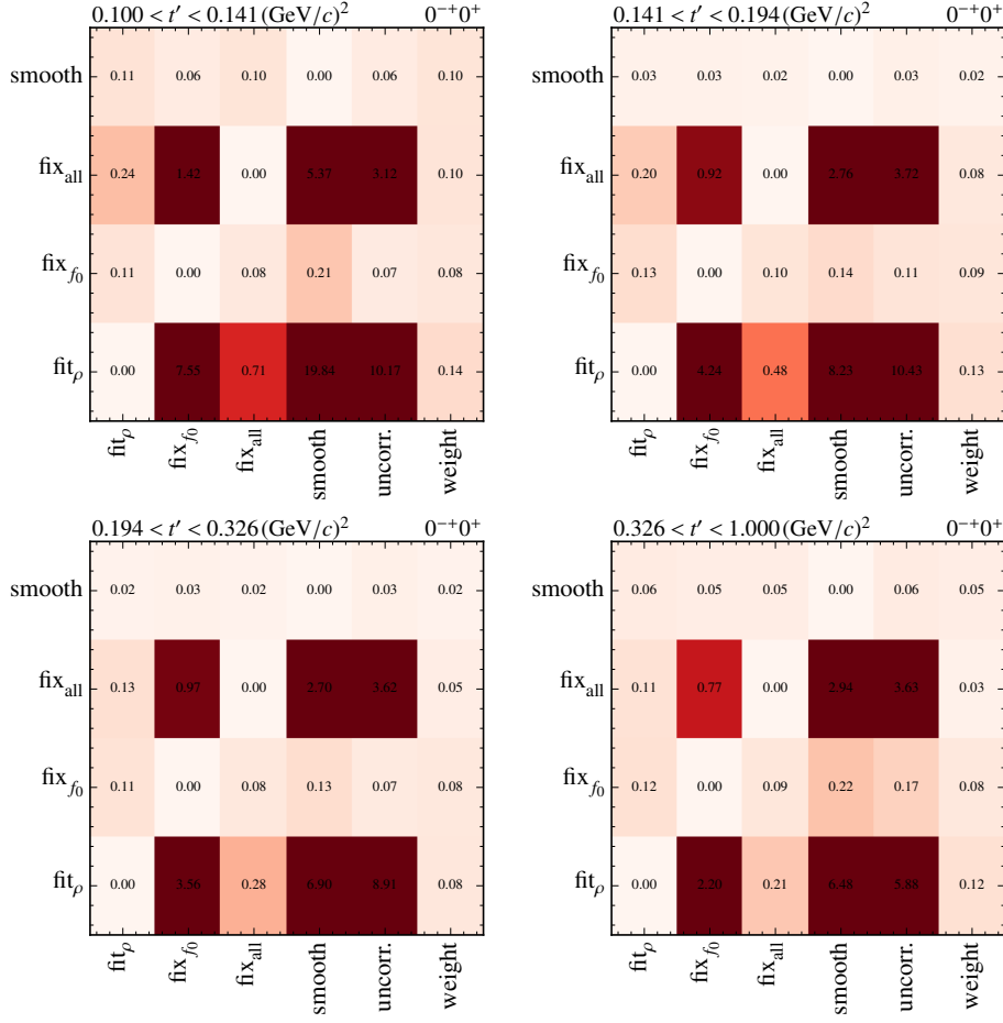
Figure 6.10.: Relative consistencies d_b^a , as defined in eq. (6.8), for the different methods to resolve the zero-mode coefficients in the J_X^{PC} M^\pi = 0^{-+}0^{+} sector for the four t' bins.
