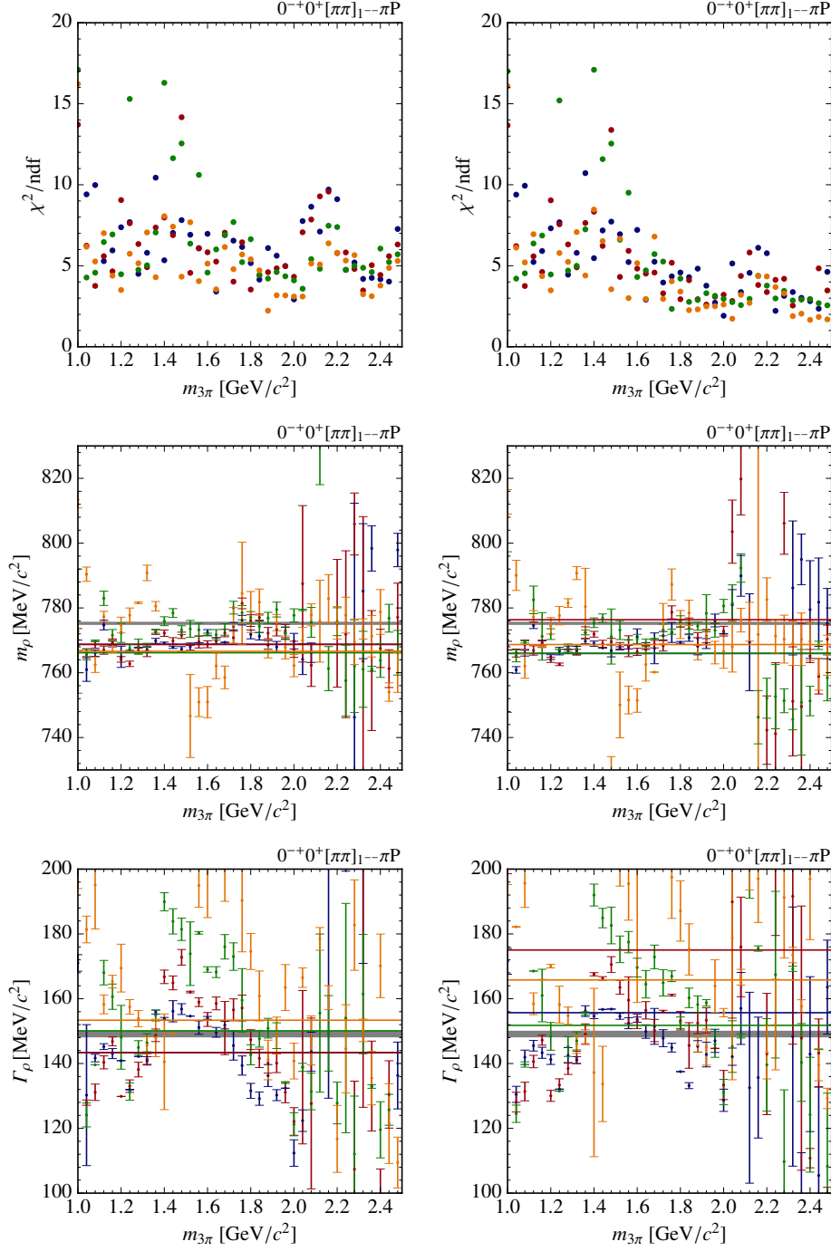
Figure 7.2.: Results of the fits in m_{3\pi} and t' bis of the isobar dynamic amplitude extracted for the 0^{-+}0^{+}[\pi\pi]_{1--}\pi P wave: The \chi^2/\text{ndf} of the fits (top), the resulting \rho(770) mass (center), and the resulting \rho(770) width (bottom). The m_{2\pi} fit range is given by kinematic limits (left) and limited to the range below 1.2 GeV/c 2 (right). The horizontal lines indicate the result of a combined fit of the \rho(770) parameters over the whole m_{3\pi} range. The colors represent different t' bins (see text). The gray band indicates the corresponding value given by the PDG [2].
