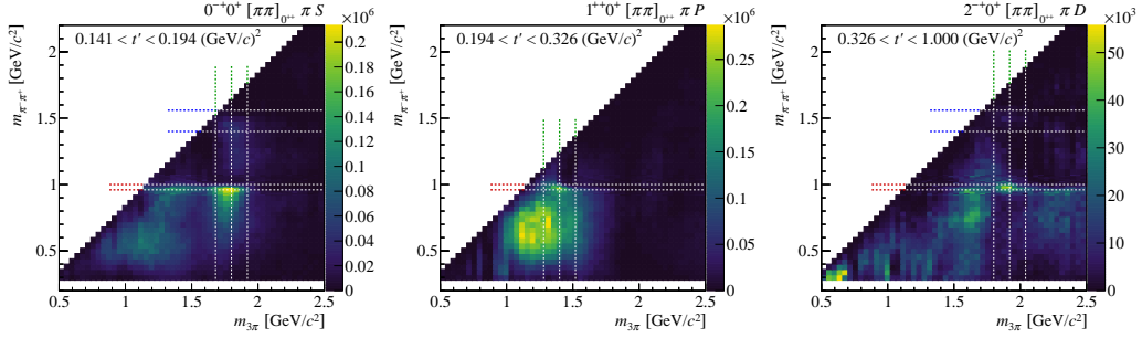
Figure 6.21.: Two dimensional intensity distribution for the 0^{-+}0^{+}[\pi\pi]_{0^{++}}\pi S wave in the second t' bin (left), for the 1^{++}0^{+}[\pi\pi]_{0^{++}}\pi P wave in the third t' bin (center), and the 2^{-+}0^{+}[\pi\pi]_{0^{++}}\pi D wave in the highest t' bin (right) taken from ref. [12].
