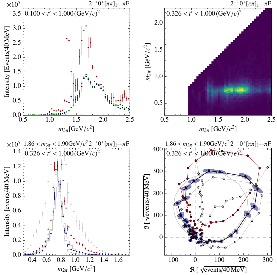
Figure 6.19.: Similar to fig. 6.11, now showing results for the 2^{-+}0^{+}[\pi\pi]_{1--}\pi F wave.
