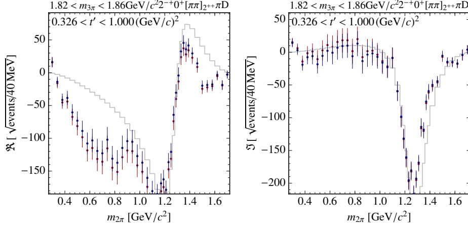
Figure 6.29.: Similar to fig. 6.28, now showing real and imaginary part of the dynamic isobar amplitude of the 2^{-+}0^{+} [\pi\pi]_{2^{++}} \pi D wave.
