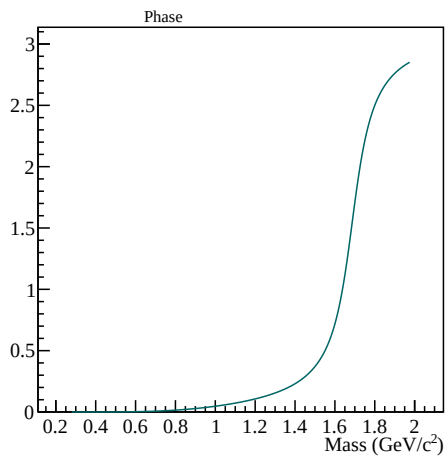
Figure C.12 Parametrisation of the \rho_3(1690) amplitude.
