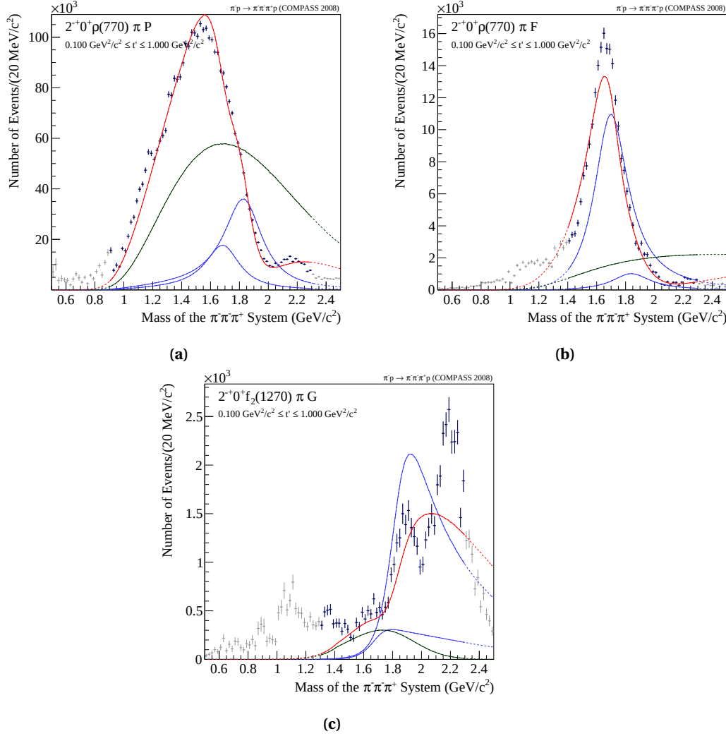
Figure 8.19 Additional fit results for 2^{-+}0^{+} partial waves based on the model listed in Tab. 8.8. The t' -integrated intensity of the 2^{-+}0^{+}\rho\pi P wave is shown in (a) with the blue markers being the data points of the spin parity analysis. The red curve showing the overall fit result, the blue curves the Breit-Wigner components and the green line the non-resonant contribution. The t' -integrated intensity of 2^{-+}0^{+}\rho\pi F wave is shown in (b) and of the 2^{-+}0^{+}f_2(1270)\pi G wave in (c)
