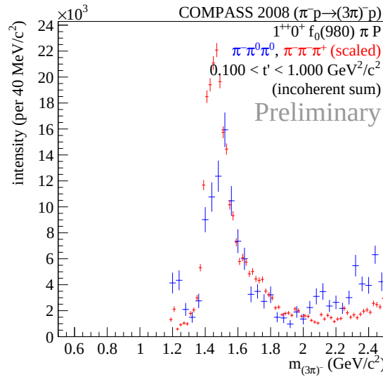
Figure 9.1 Intensity of the 1^{++}0^+f_0(980)\pi P wave for the charged and neutral final state overlaid. The intensity of the charged channel is scaled to the intensity of the neutral channel in order to compare the line shape. Plot from [Uhl14].
