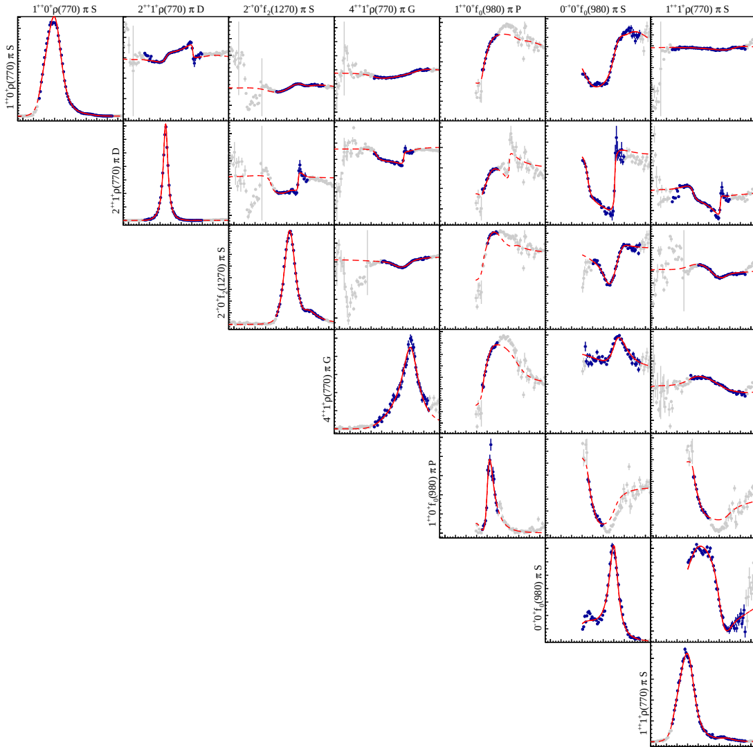
Figure 8.2 Spin-density matrix \rho(m_{\pi\pi}, t') with the fit result of the model listed in Tab. 8.2 in the bin of 0.144 \leq t' \leq 0.164 \text{ GeV}^2/c^2 .
