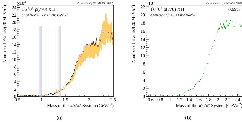
Figure 7.8 Integrated intensity of the partial wave with J^{PC} M^z \pi L = 6^{-+} 0^+ \rho(770) \pi H (a). This amplitudes is assumed to be dominated by Deck-produced final states and thus is taken as normalisation for the fit results of the Deck Monte Carlo data sample (b). The yellow band in plot (a) shows the maximum spread of the intensity with respect to the systematic studies, discussed in Sec. 7.6. The blue lines corresponds to thresholds applied to some amplitudes.
