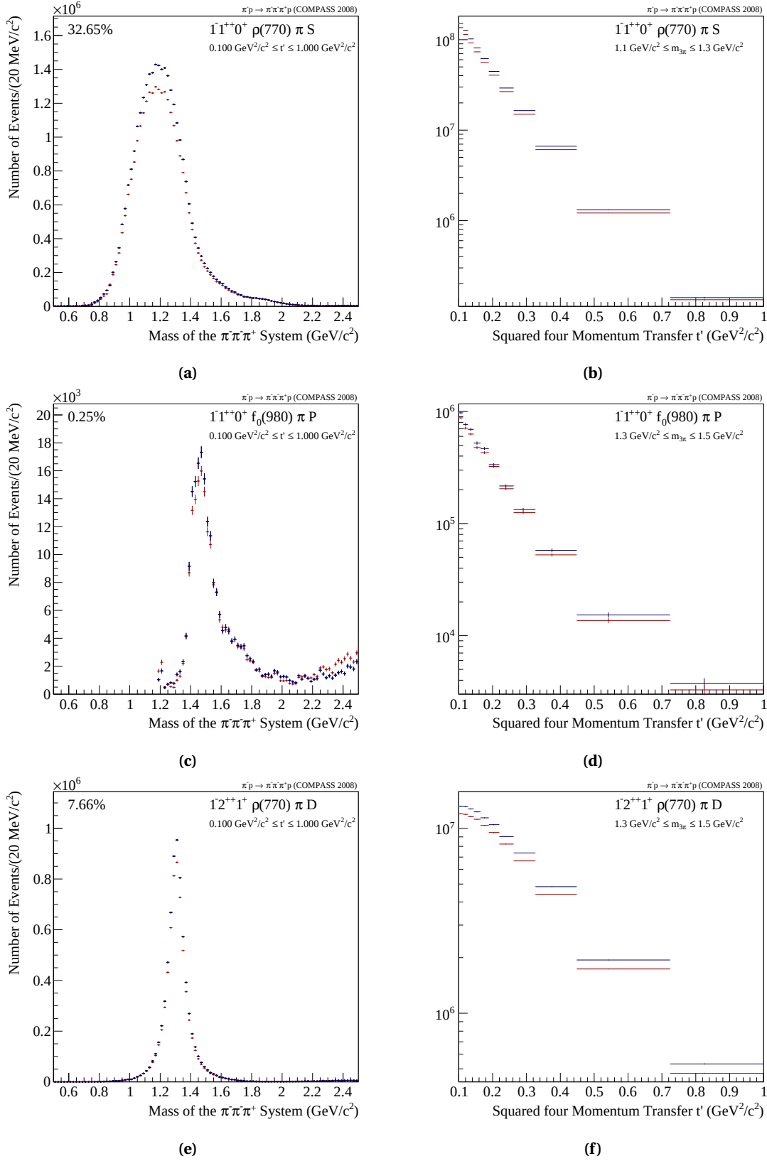
Figure 7.41 Integrated intensity of the 1^{++}0^+ \rho\pi S wave obtained from the main fit (blue) overlaid by the normalised fit result based on a data sample with looser cuts (red) (a), the corresponding t' dependence (b). The same plot for the new a_1 state (c) and (d) and the 2^{++}1^+ \rho\pi D wave (e) and (f).
