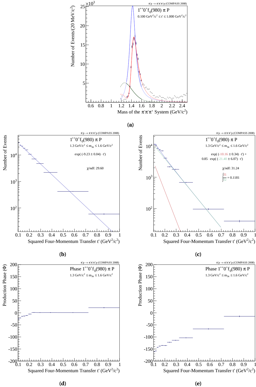
Figure 8.5 Fit result for the 1^{++}0^+ f_0(980) \pi P partial wave based on the model listed in Tab. 8.2. The t' -integrated intensity is shown in (a) with the blue markers being the data points of the spin-parity analysis. The red curve shows the overall fit result, the blue curves the Breit-Wigner components and the green line the non-resonant contribution. The t' dependence of the a_1(1420) is plotted in (b) and that of the non-resonant contribution in (c). The corresponding production phases are shown in (d) and (e).
