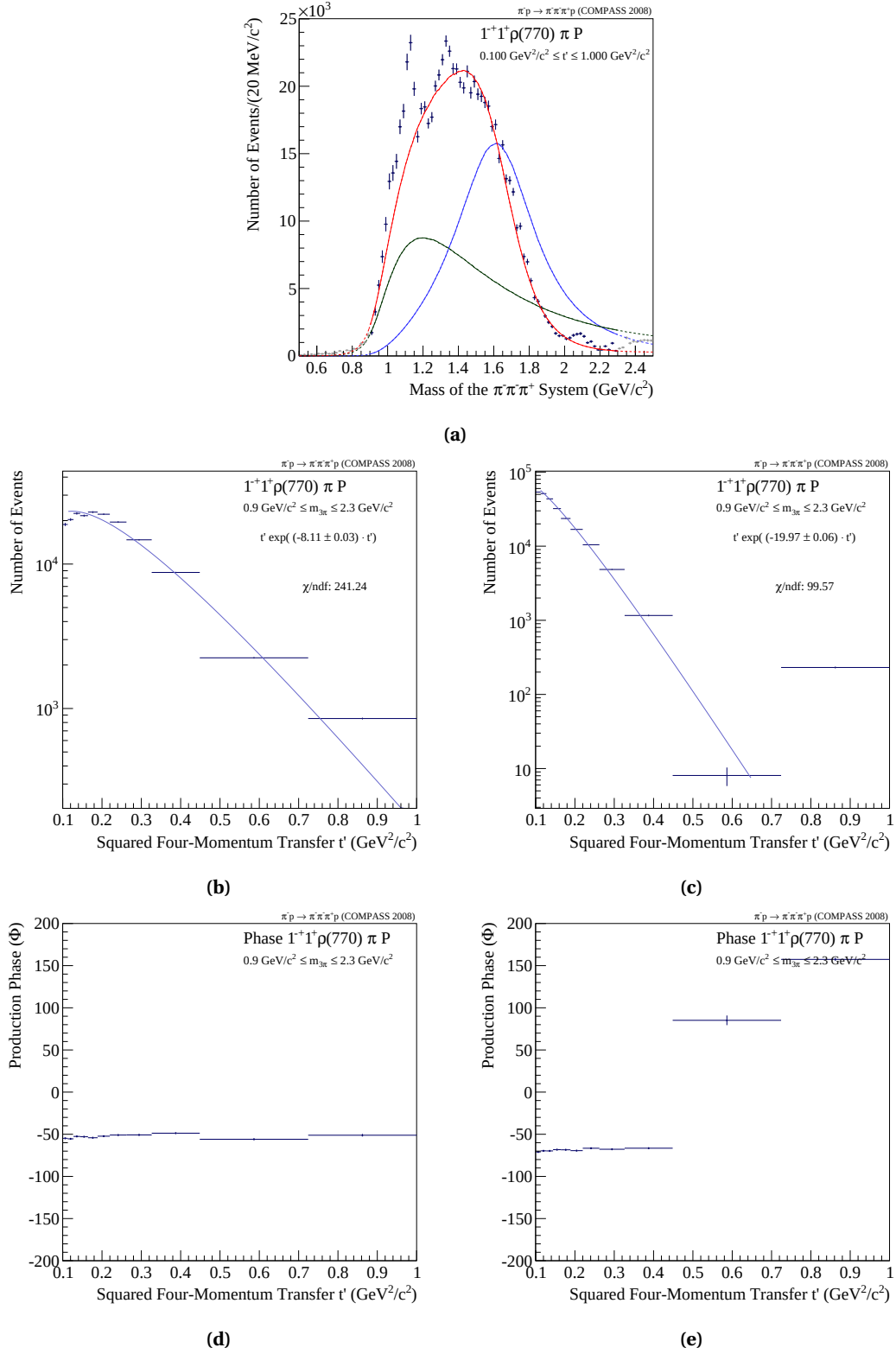
Figure 8.10 Fit result for the partial wave 1^{-+}1^{+}\rho\pi P based on the model listed in Tab. 8.4. The t' integrated intensity is shown in (a) with the blue markers being the data points of the spin-parity analysis. The red curve is showing the overall fit result, the blue curves the implemented Breit-Wigner components and the green line shows the non-resonant contribution. The t' dependence of the \pi_1(1600) is plotted in (b) and the t' dependence of the non-resonant contribution in (c). The corresponding production phases are shown in (d) and (e).
