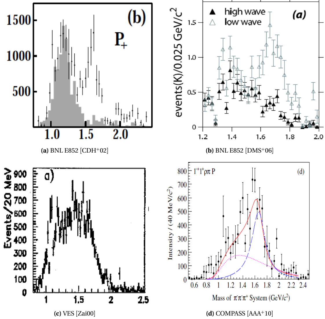
Figure 1.3 Overview of analyses investigating the spin-exotic 1^{-+} in the \pi^{-}\pi^{-}\pi^{+} channel.
