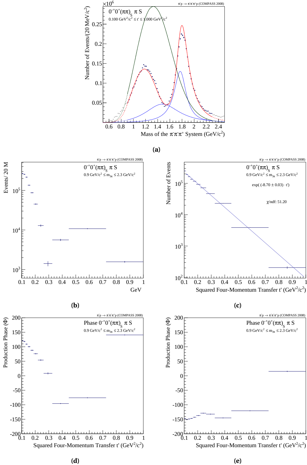
Figure 8.13 Fit result for the 0^{-+}0^{+}(\pi\pi)_S \pi S partial wave based on the model listed in Tab. 8.6. The t' -integrated intensity is shown in (a) with the blue markers being the data points of the spin-parity analysis. The red curve shows the overall fit result, the blue curves the Breit-Wigner components and the green line the non-resonant contribution. The t' dependence of the \pi(1300) is plotted in (b) and that of the \pi(1800) in (c). The corresponding production phases are shown in (d) and (e).
