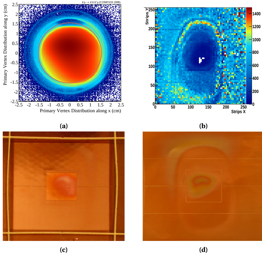
Figure 4.10 The beam shape seen in reconstructed 3\pi data (a), aging observed on the readout foil of P03XY (c). Cluster amplitude in arbitrary units (b) and aging observed on the bottom side of the third EM foil, both for GP03XY. Plots (b), (c) and (d) from [Tas11].
