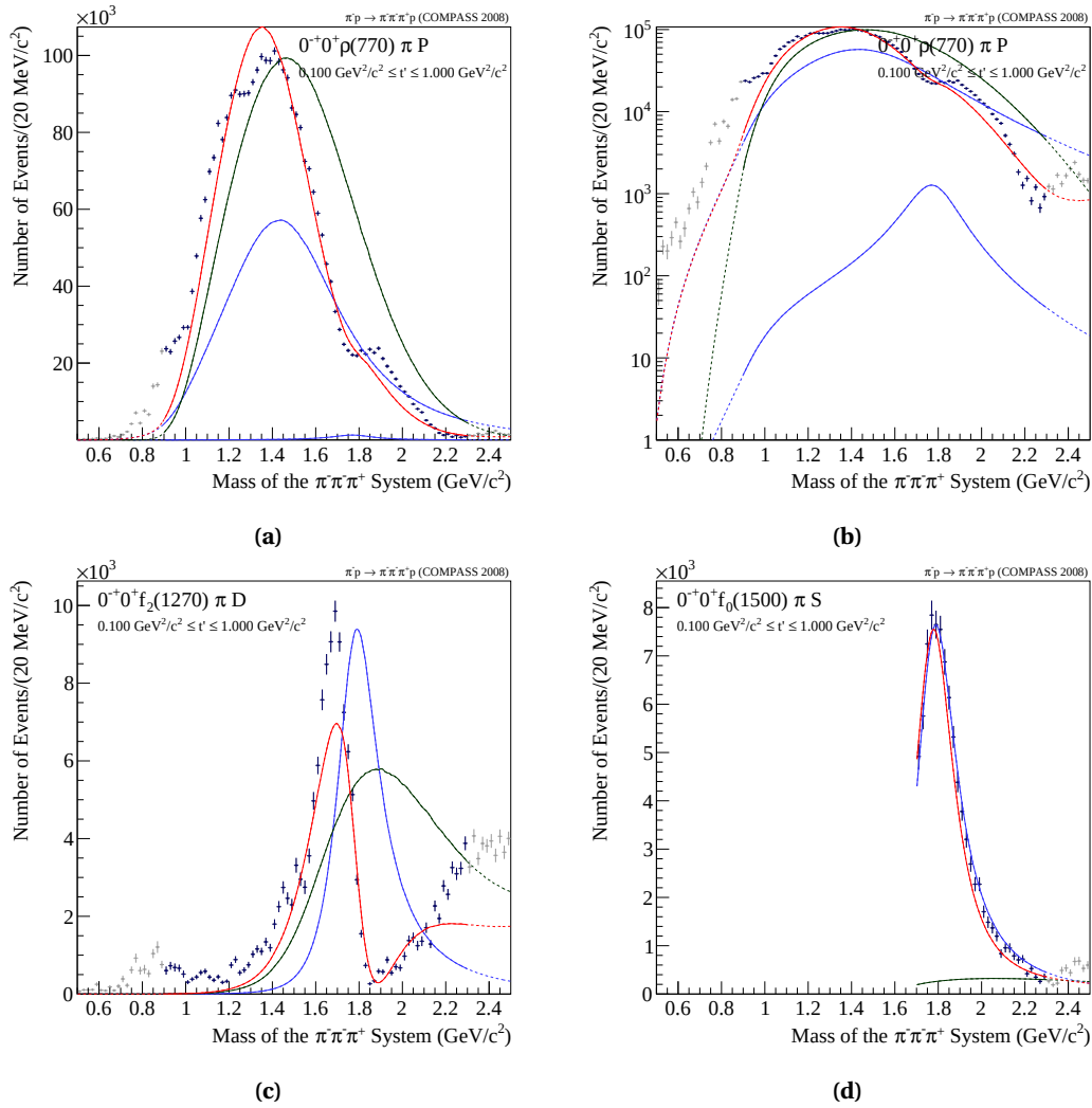
Figure 8.14 Additional fit results for 0^{-+}0^{+} partial waves based on the model listed in Tab. 8.6. The t' -integrated intensity of the 0^{-+}0^{+}\rho\pi P wave is shown in (a) with the blue markers being the data points of the spin-parity analysis. The red curve is showing the overall fit result, the blue curves the Breit-Wigner components and the green line shows the non-resonant contribution. The same plot in a logarithmic scale where the second Breit-Wigner is visible (b). The t' -integrated intensity of 0^{-+}0^{+}f_2(1270)\pi D wave is shown in (c) and that of the 0^{-+}0^{+}f_0(1500)\pi S wave in (d)
