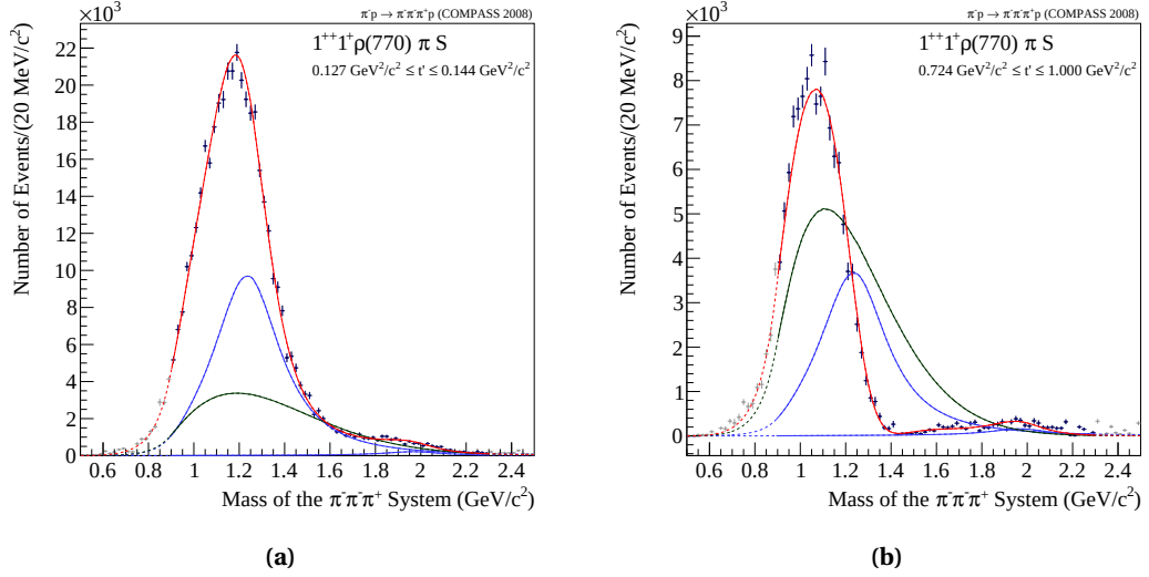
Figure F.4 Fit result for the 1^{++}1^+\rho\pi S partial wave based on the model listed in Tab. 8.2 for selected t' bins.
