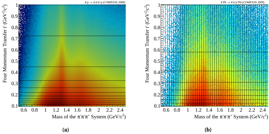
Figure 7.7 Binning of the kinematic range of the invariant mass m_{3\pi} and the squared four-momentum transfer t' . Equidistant mass bins are chosen (20 \text{MeV}/c^2 ) with 11 t' bins (a) or (40 \text{MeV}/c^2 ) with 8 t' bins (lead data) (b).
