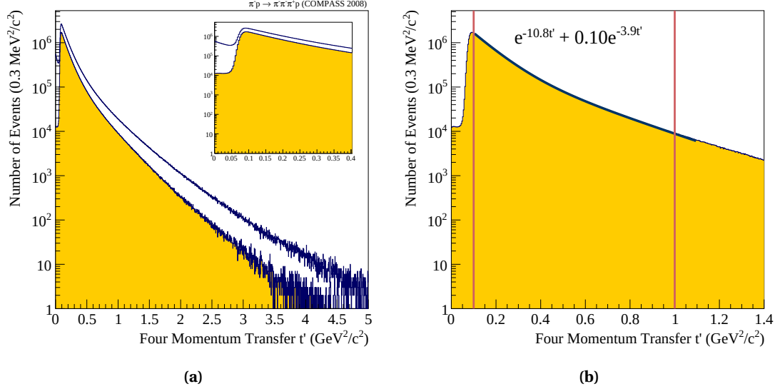
Figure 5.8 Figure (a) shows the t' distribution without (open histogram) and with (filled histogram) coplanar cut applied. The kinematical boundaries of the analysis are depicted in Fig. (b), denoted by red lines. All plots have logarithmic scale.
