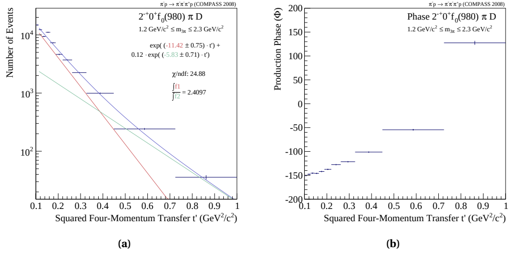
Figure E.10 Fit result for the 2^{-+}0^{+}f_0(980)\pi D partial wave based on the model listed in Tab. 8.8. The t' dependence of the non-resonant is shown in (a) and the corresponding production phase (b).
