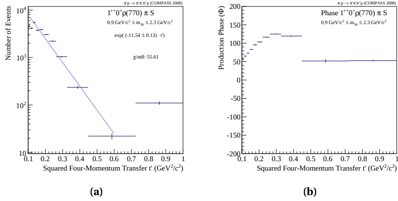
Figure F.1 Fit result for the 1^{++}0^+\rho\pi S partial wave based on the model listed in Tab. 8.2. The t' dependence of the a_1(1910) is shown in (a) and the corresponding production phase (b).
