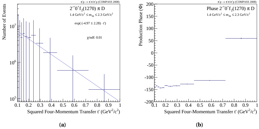
Figure F.9 Fit result for the 2^{-+}0^{+}f_2(1270)\pi D partial wave based on the model listed in Tab. 8.8. The t' dependence of the non-resonant is shown in (a) and the corresponding production phase (b).
