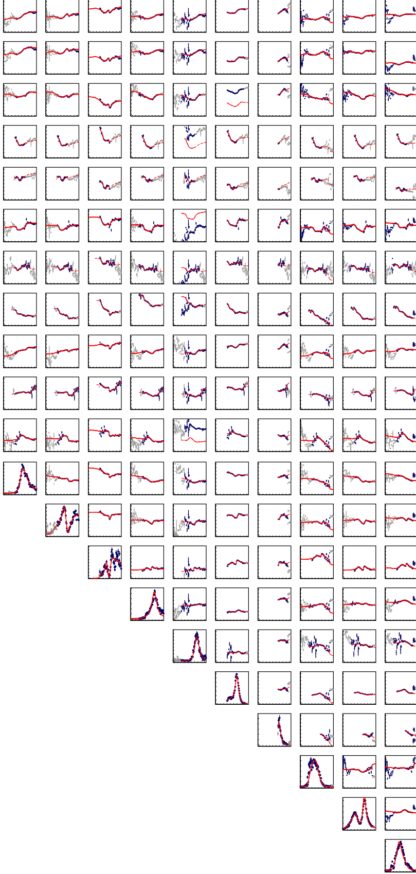
Figure 9.3 Spin-density matrix \rho(m_x) of a model consisting of 21 partial waves in the kinematic region of 0.164 \leq t' \leq 0.189 \text{ GeV}^2/c^2 .
