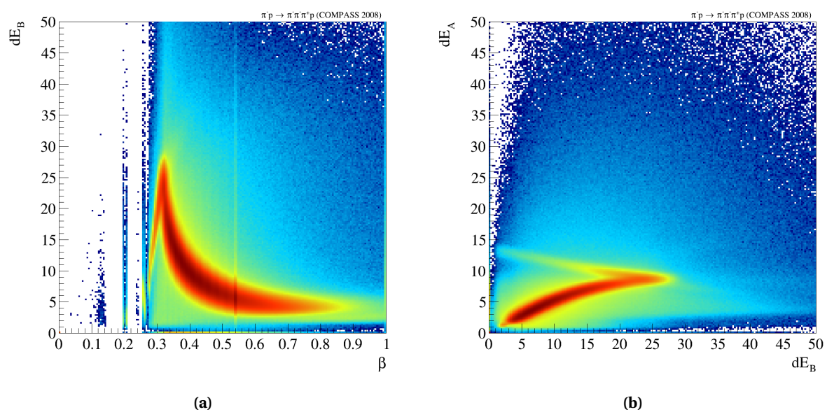
Figure A.7 Energy loss in the RPD.
