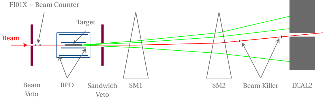
Figure 5.3 Trigger scheme of the DT0 trigger: The main component is the RPD detector (blue), triggering on slow charged particles leaving the target. In addition the alternative beam trigger (blue) is tagging single incoming beam particles. The veto system (violet), consisting of beam veto, sandwich and beam killer, is completing the DT0 trigger system.
