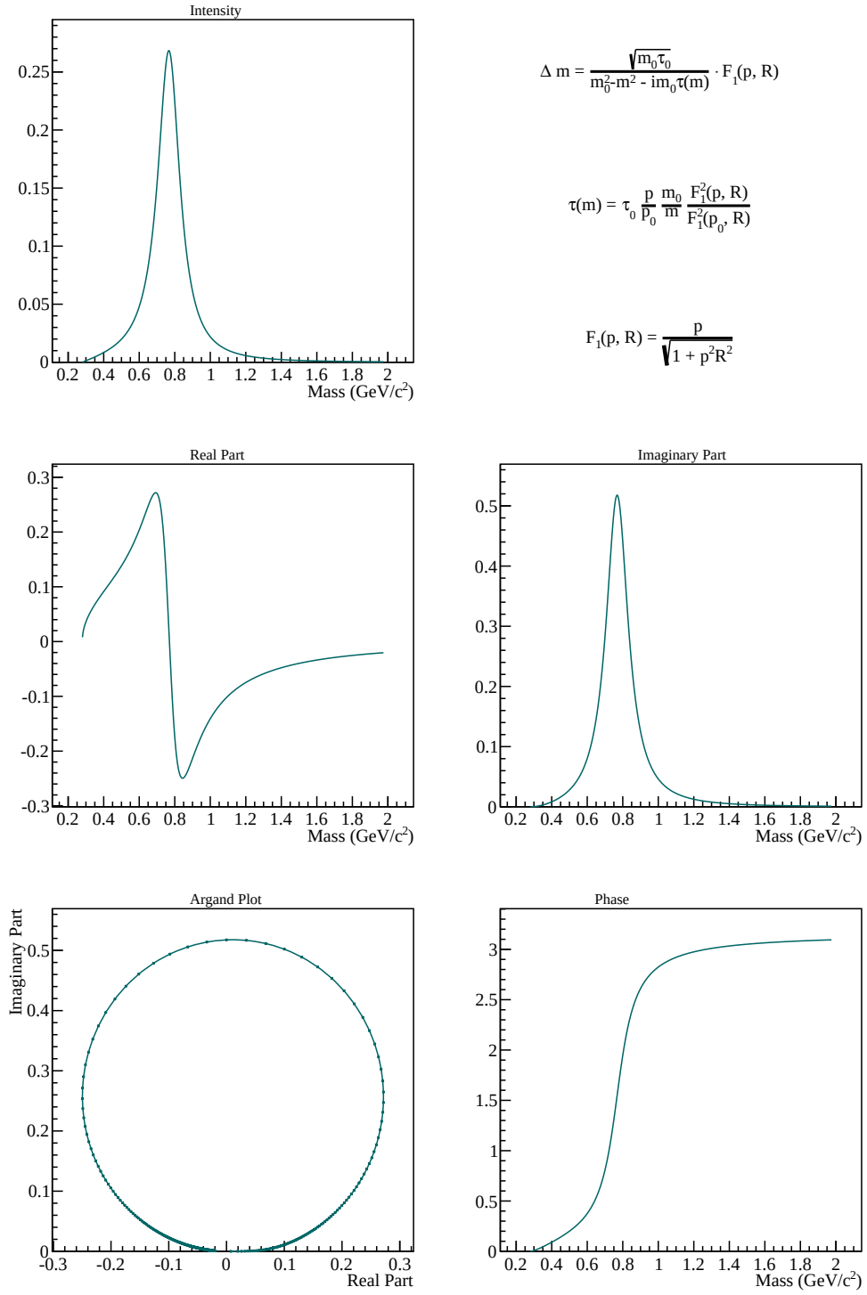
Figure C.9 Parametrisation of the \rho(770) .
