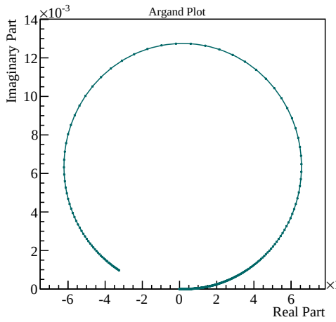
Figure C.12 Parametrisation of the \rho_3(1690) amplitude.
