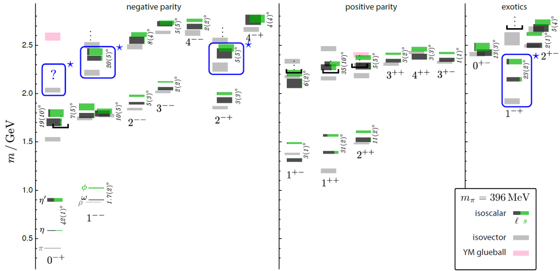
Figure 1.2 Spectrum of isoscalar and isovector mesons obtained by LQCD, plot from [Dud11].
