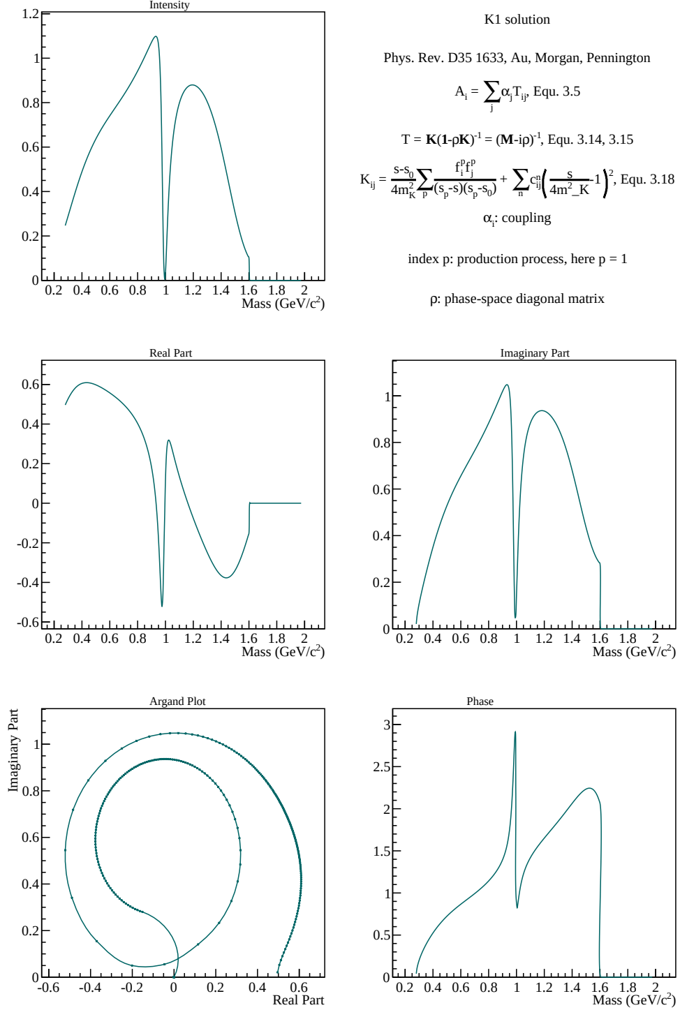
Figure C.1 (\pi\pi)_S wave parametrisation. Based on the 'K1'-solution, described in [AMP87].
