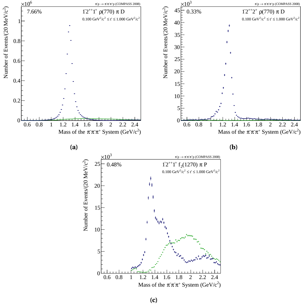
Figure 7.15 Integrated intensity of partial waves with J^{PC} = 2^{++} decaying into the \rho(770) isobar, with spin projection M^E = 1^+ (a) and M^E = 2^+ (b) and decaying into f_2(1270) shown in (c).
