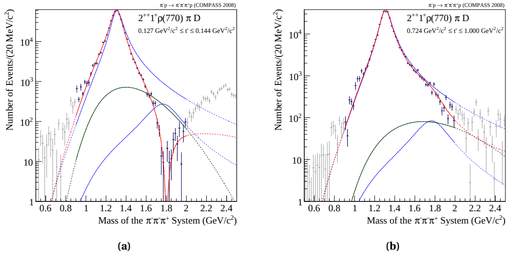
Figure F.5 Fit result for the 2^{++}1^+\rho\pi D partial wave based on the model listed in Tab. 8.4 for selected t' bins.
