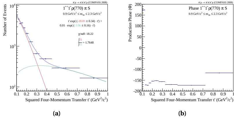
Figure F.2 Fit result for the 1^{++}1^+\rho\pi S partial wave based on the model listed in Tab. 8.2. The t' dependence of the a_1(1910) is shown in (a) and the corresponding production phase (b).
