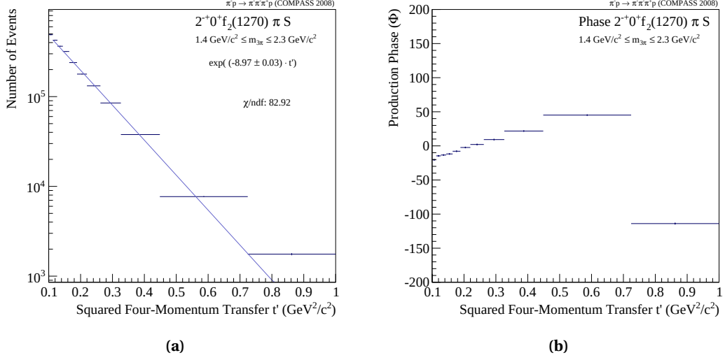
Figure F.8 Fit result for the 2^{-+}0^{+}f_2(1270)\pi S partial wave based on the model listed in Tab. 8.8. The t' dependence of the non-resonant is shown in (a) and the corresponding production phase (b).
