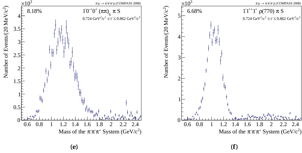
Figure 7.25 Intensity of the 0^{-+}0^{+}(\pi\pi)_{\text{S}}\pi\text{S} wave for increasing t' regions (a), (c) and (e) and accordingly for the 1^{-+}1^{+}\rho\pi\text{S} wave (b), (d) and (f).
