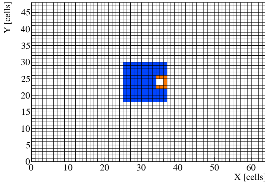
Figure 34: The active area of the ECAL2 trigger (shown in blue). The cells shown in orange are rejected due to high rates.
