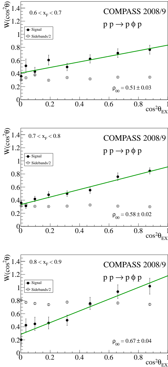
Figure 71: Angular distributions (full circles) with respect to the direction of momentum transfer for \phi . The panels show different x_F regions: 0.6–0.7 (upper panel), 0.7–0.8 (middle panel) and 0.8–0.9 (lower panel). The open circles show the background distribution in the sidebands.
