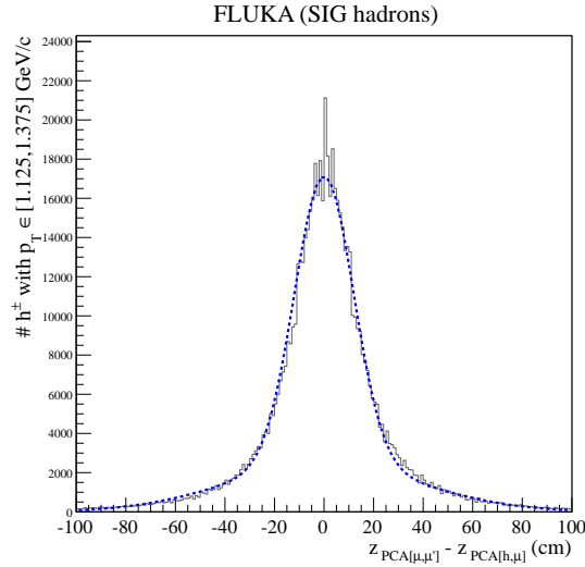
Figure B.3: Distribution of D (Eq. (6.3)) for signal hadrons from the simulation with FLUKA. The distribution is fitted with the function f_{\text{SIG}} (Eq. (6.4)), which is centered at zero. [referenced from 6.3.2 (p. 80)]
