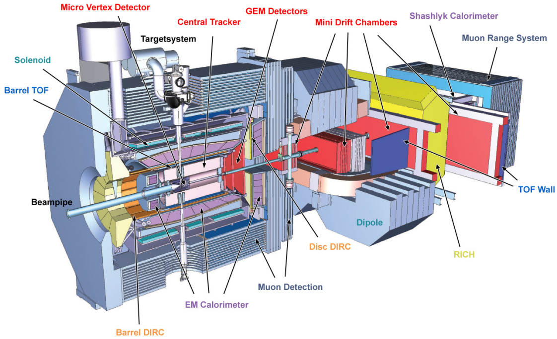
Figure 7.4: Schematic view of the \bar{\text{P}}\text{ANDA} spectrometer, which has an overall length of \sim 12 m.
