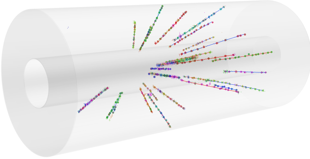
Figure 8.11: Visualization of a ^{22}\text{Ne} -Al event in the TPC. The Riemann pattern recognition described in Sec. 8.6 has been used to identify the individual particle tracks, as indicated by the lines.
