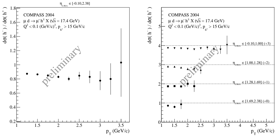
(c) Charge ratio of cross section integrated over \eta_{c.m.s.} .
