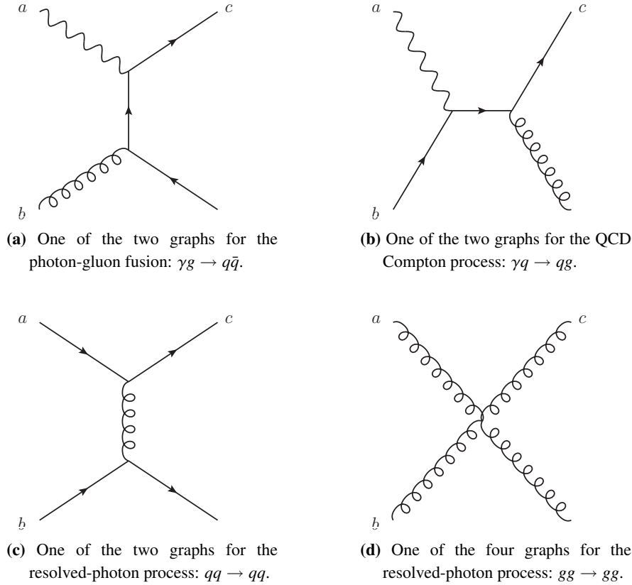
Figure 3.2: Examples of the leading-order Feynman graphs of the partonic cross sections, \hat{\sigma}_{ab \rightarrow cX} , for high- p_T scattering of Fig. 3.1.
