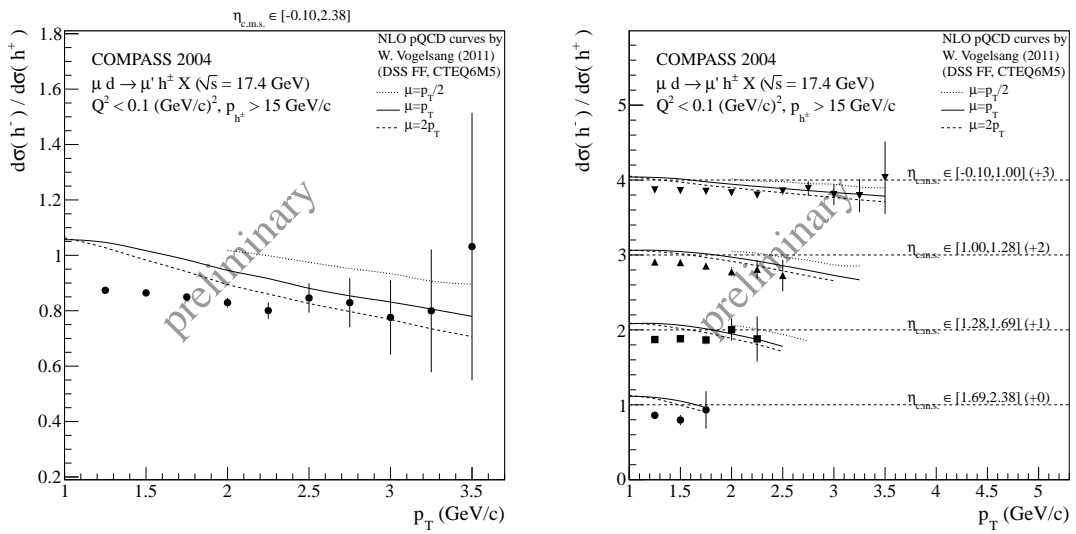
(d) Charge ratio of cross section integrated over \eta_{c.m.s.} . (e) Charge ratio of cross section binned in \eta_{c.m.s.} . Please note that the graphs are offset by constants, as indicated on the right (dashed lines indicate ratios of one).
