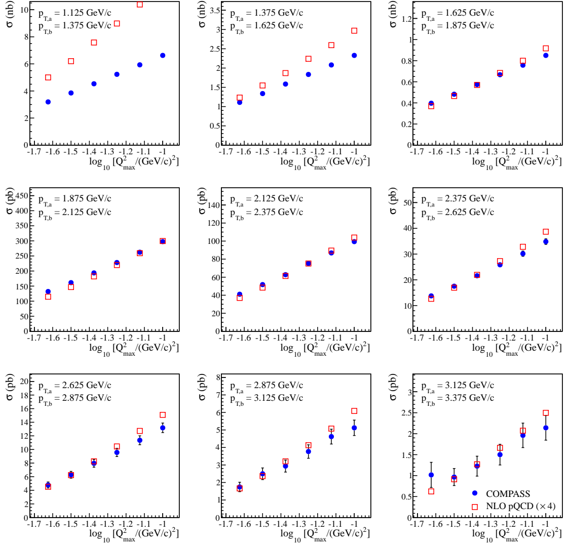
Figure 6.24: Comparison of the Q_{\max}^2 dependence of the COMPASS and the NLO pQCD cross sections in p_T bins. The theory cross sections have been computed for this work by W. Vogelsang [37] and are scaled up by an arbitrary factor of four to allow a better comparison of the Q_{\max}^2 slopes. The error bars of the COMPASS data points are purely statistical.
