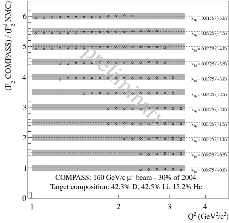
Figure 5.16: Comparison of the structure function F_2 extracted from COMPASS data with the parametrization from NMC [88]. The ratios for the individual x_{\text{Bj}} bins are offset by constant factors as indicated on the right hand side of the plot. The gray bands indicate the 10% normalization uncertainty arising from the systematic error of the luminosity. All values lie within the bands, thus proving consistency with the NMC result.
