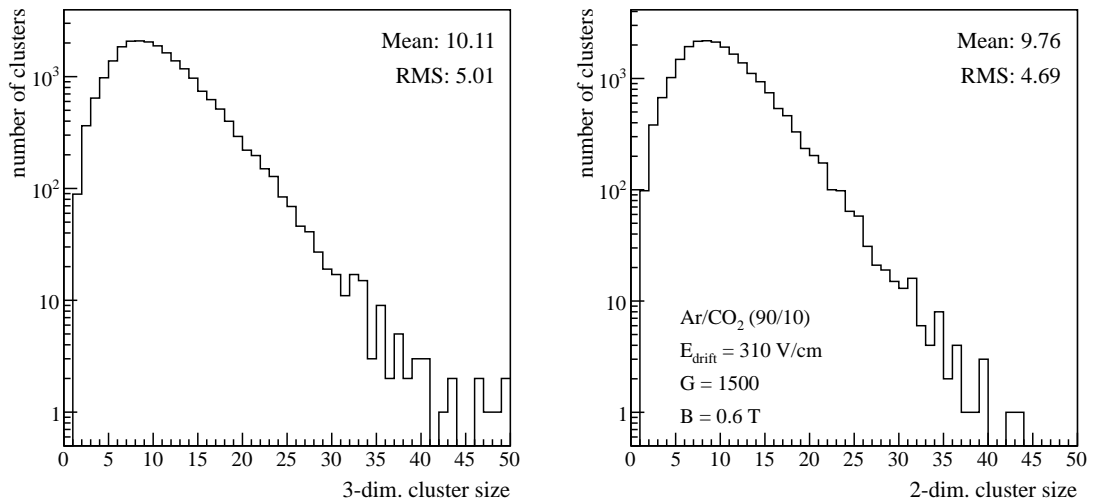
Figure 8.16: Cluster-size distributions for cosmic-muon tracks that are traversing the detector almost parallel to the pad plane. For the definitions of the 3-dim. (left) and 2-dim. (right) cluster sizes, see text.
