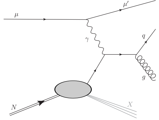
Figure 2.4: Feynman graph of lepton-quark scattering with the emission of a hard gluon.
