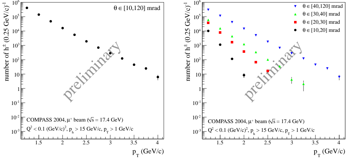
Figure 6.1: Yield of charged hadrons h^\pm with high p_T . The left plot presents the data integrated over the full \theta range, whereas the right plot is binned in \theta (definition of \theta in the text).
