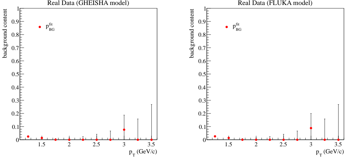
Figure 6.14: Summary of the background contents determined by the f_{i,ALL} fits to the real data with the GHEISHA model (Fig. 6.13) and the FLUKA model (Fig. B.7).
