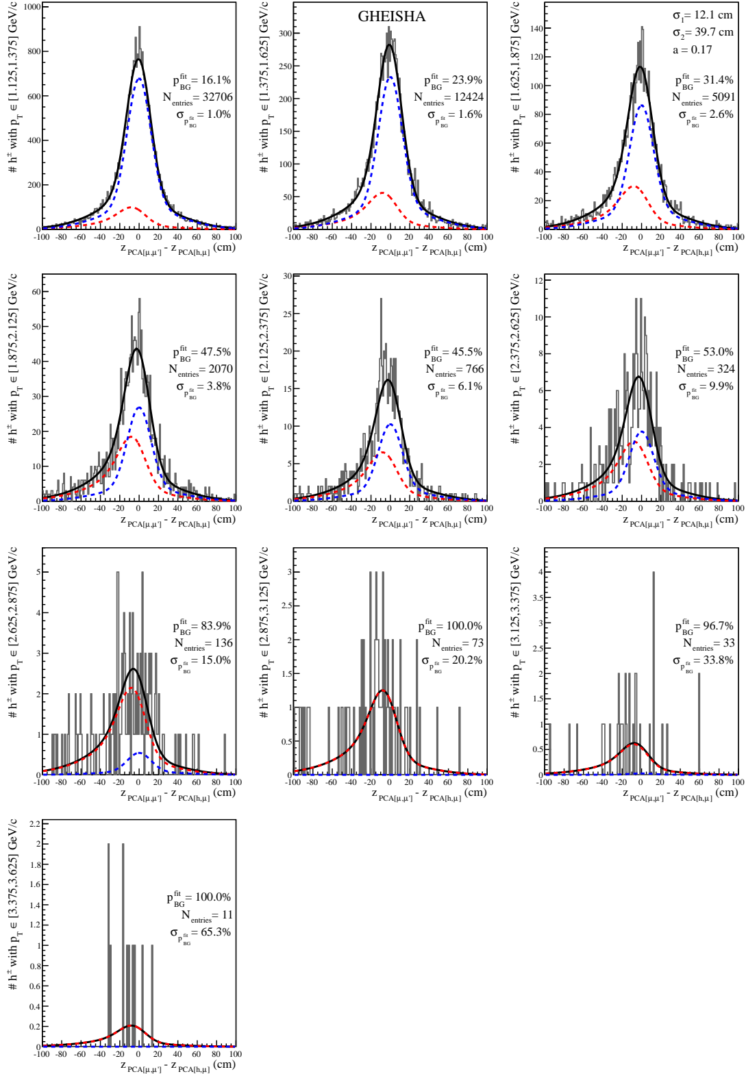
Figure 6.11: Distributions of D for all hadrons from the simulation with GHEISHA in bins of p_T .
