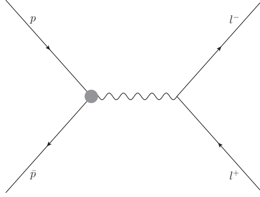
Figure 7.2: \bar{p}p annihilation into l^+l^- to investigate the time-like form factors of the proton.
