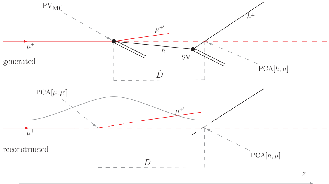
Figure 6.7: Definition the variables \tilde{D} and D for an event with a secondary interaction. The upper sketch shows the generated event topology, while the lower sketch illustrates the reconstructed event topology.
