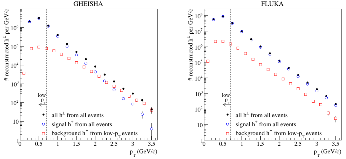
Figure 6.6: Contributions of primary hadrons (signal, blue circles) and misreconstructed secondary hadrons from low- p_T events (background, red squares) to the overall hadron yield (black filled circles) in simulations based on GHEISHA (left plot) and FLUKA (right plot). Low- p_T events are defined as events that do not have any charged hadrons with p_{T,\text{gen}} > 0.7 \text{ GeV}/c .
