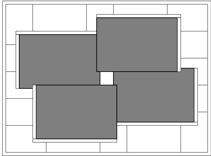
Figure 3.2: Geometry with 4 identical modules around the beam hole.
