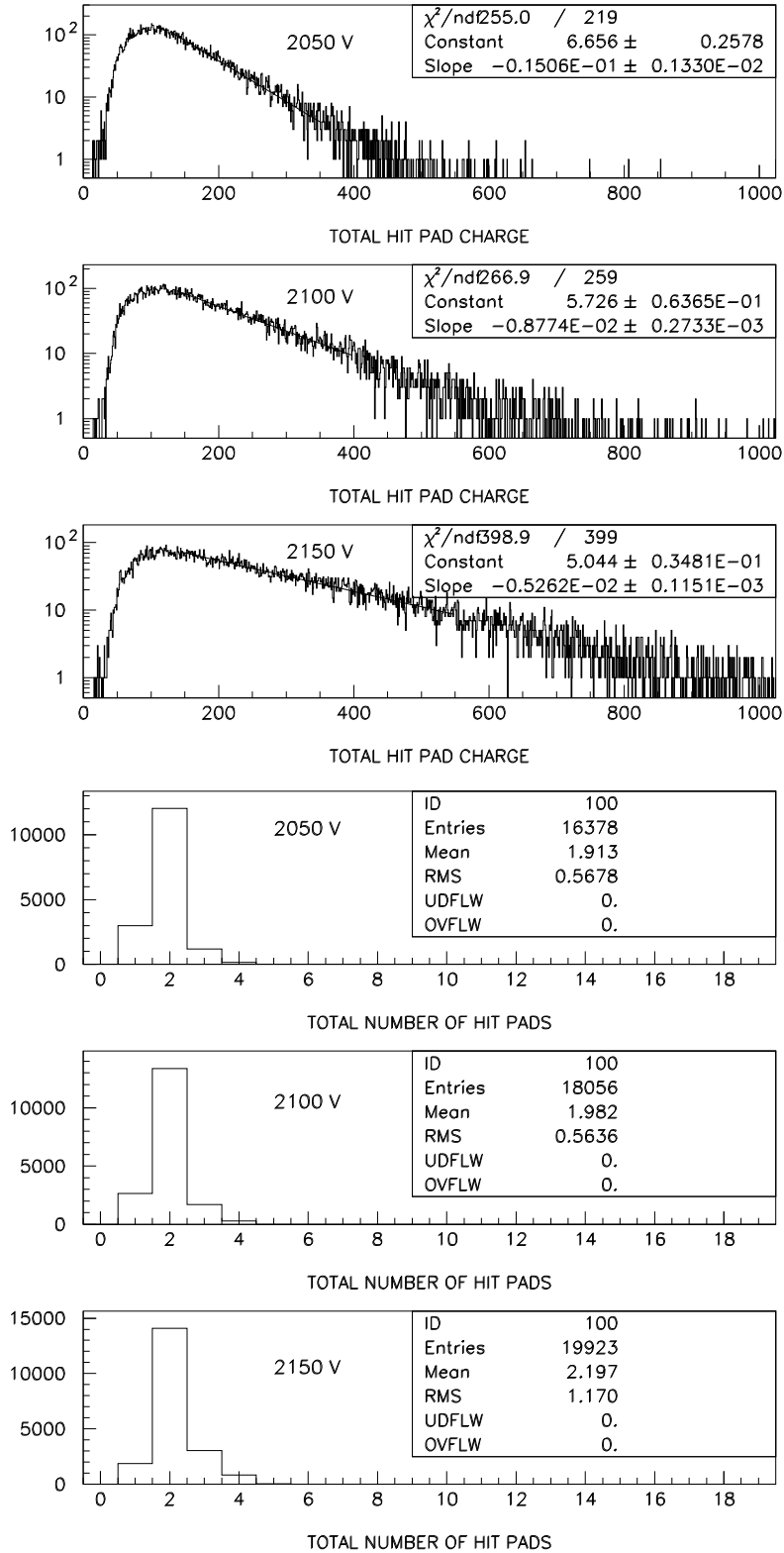
Figure 3.3: Results of tests on the photon detector prototype, using a UV lamp and a pad cathode plane without the CsI deposit: a) Spectra of signal amplitude for single photon detection; the efficiency for single photo-electron detection is 90% at 2100 V. b) Distribution of the number of cathode pads giving signal above threshold for single photon detection.
