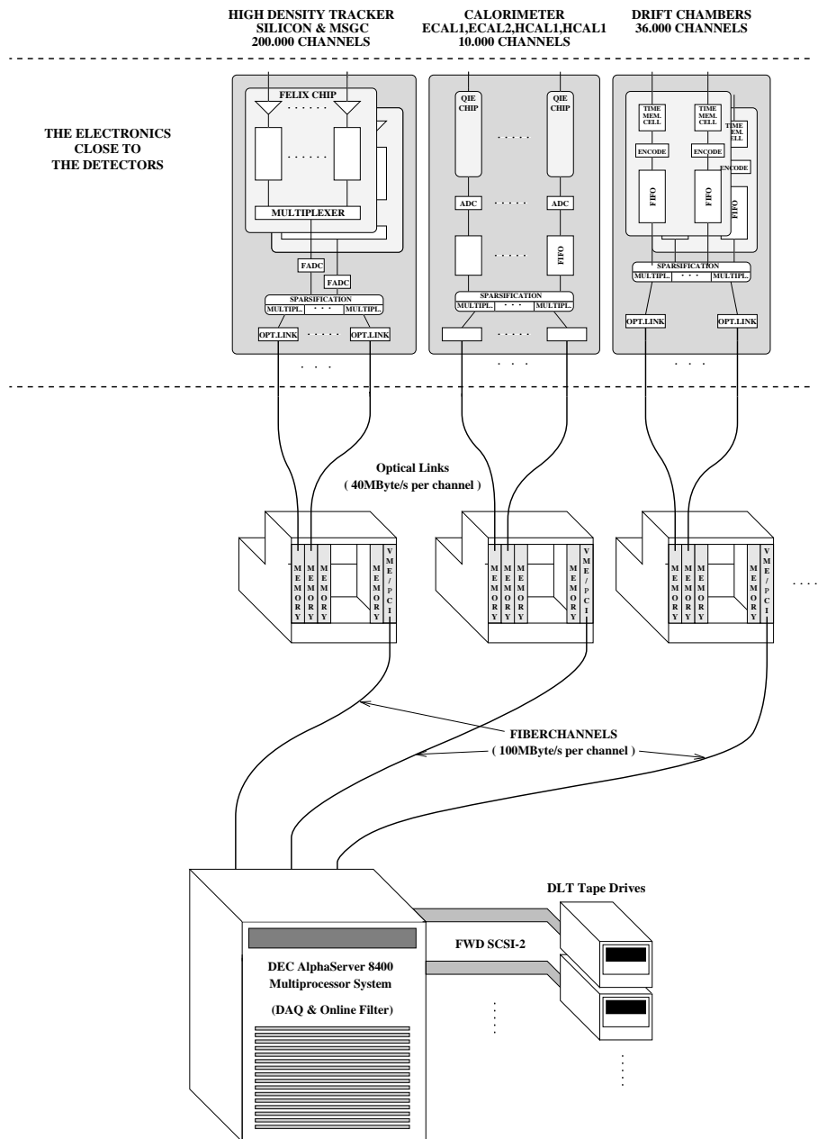
Figure 3.8: The data flow of the proposed data acquisition system. The first level consists of the frontend electronics mostly mounted close to the various detectors. The second level consists of large memory modules in VME controlled by simple processors. Master CPUs provide run control, slow control software links etc. The third level is the DAQ machine, which does event building and online filtering.
