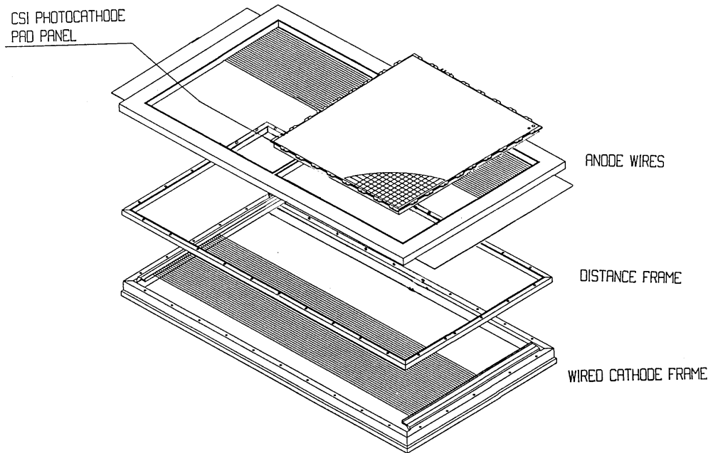
Figure 3.5: General view of the modular photon chamber ( 100 \times 60 \text{ cm}^2 )
