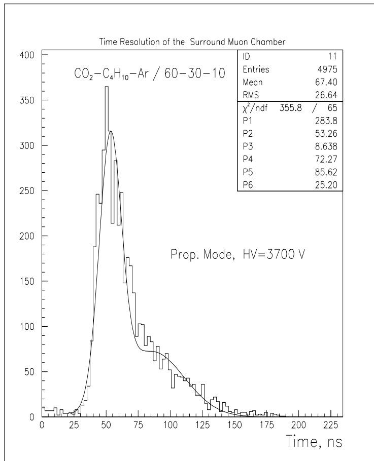
Figure 3.7: Measured time spectrum of PIT used in the DELPHI Surround Muon Chamber. 1)
