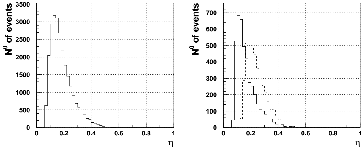
Figure 2.1: \eta distribution of gluons in open charm production: a) 35 < \nu < 85 GeV; b) dashed line 30 < \nu < 45 GeV, solid line 75 < \nu < 90 GeV.
