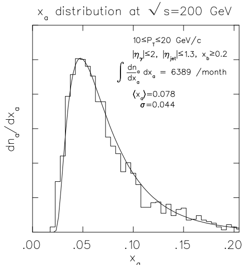
Figure 2.2: The gluon momentum fraction covered in prompt- \gamma production.
