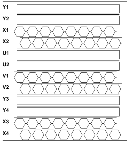
Figure 3.1: Chamber module consisting of 12 layers honeycomb cells.
