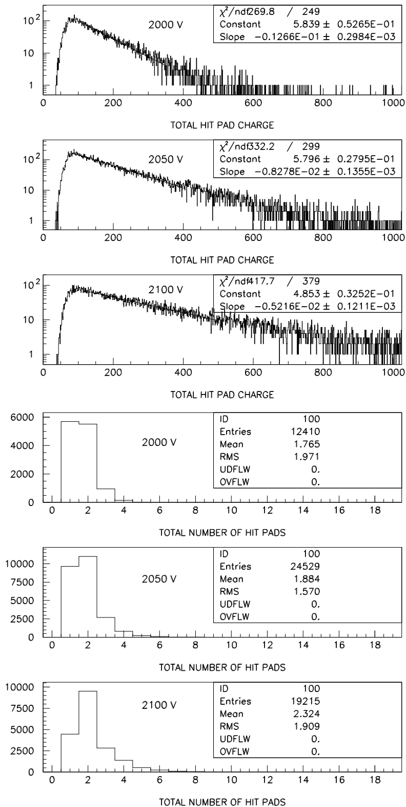
Figure 3.4: Results of tests on the photon detector prototype, using a UV lamp and a pad cathode plane with the CsI deposit: a) Spectra of signal amplitude for single photon detection; the efficiency for single photo-electron detection is 90% at 2050 V. b) Distribution of the number of cathode pads giving signal above threshold for single photon detection.
