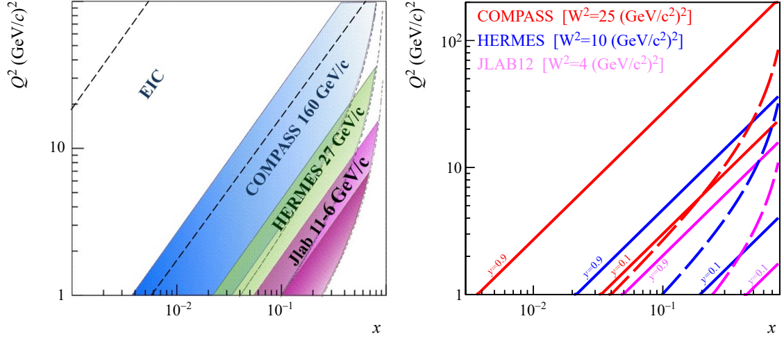
Figure 2: The x - Q^2 scatter plot for SIDIS experiments HERMES, COMPASS and JLab12. Left: also indicated with dash lines are the (\sqrt{s} = 140 \text{ GeV}, y = 0.9) and (\sqrt{s} = 40 \text{ GeV}, y = 0.1) borders for a future EIC. Only the kinematic ranges are drawn, independently of the luminosity and of the years needed to perform the measurements. Right: the full lines indicate the y = 0.1 and y = 0.9 boundaries for the three experiments, the dashed lines the corresponding W^2 values.
