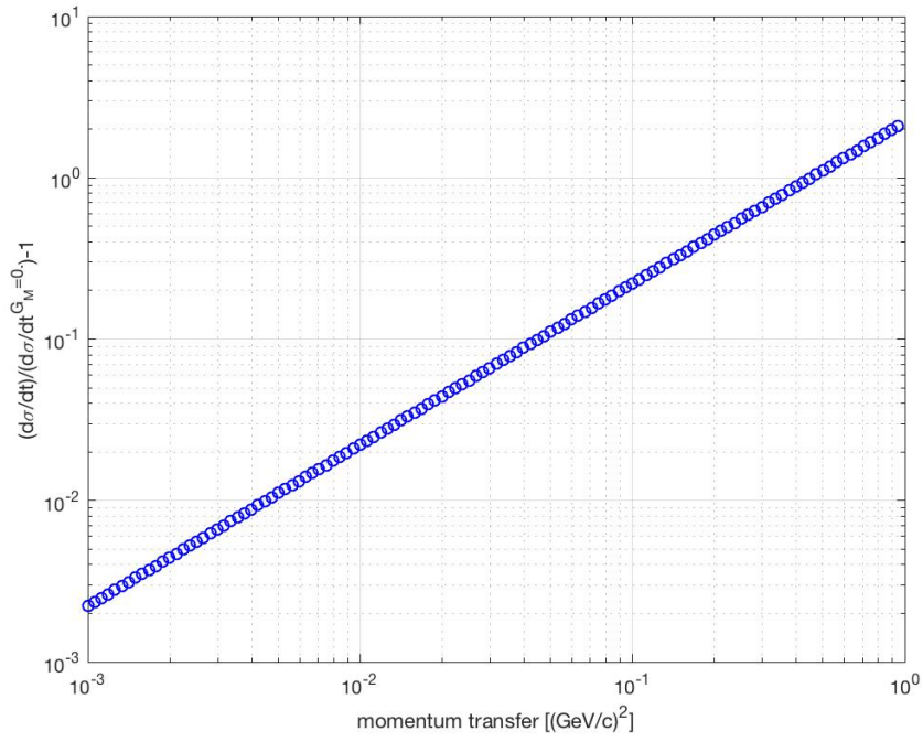
Figure 34: Relative contribution of the magnetic form factor to the elastic cross-section for different values of Q^2 . The cross-sections are evaluated using Eq. (2) with E_{beam} = 100 GeV.
