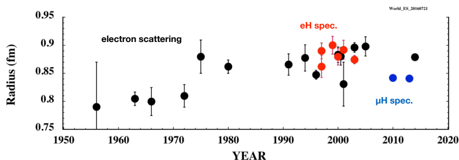
Figure 9: Historical development of the proton charge radius. Figure is taken from [41].
