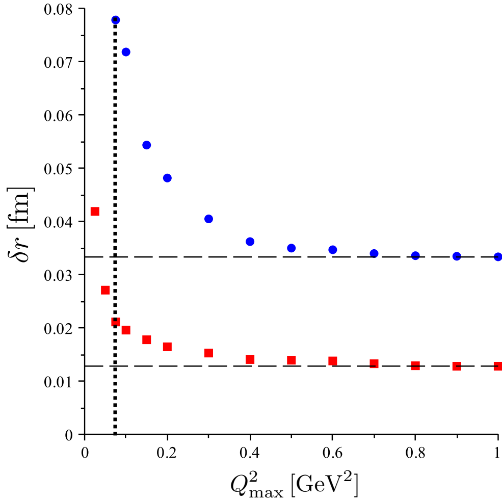
Figure 27: Statistical error on the proton charge radius as a function of the maximum momentum transfer retained in the fit, Q^2_{\max} , for the 1422 point A1 MAMI dataset (red squares) and for the complementary world cross section and polarisation dataset (blue circles). The horizontal dashed lines are large- Q^2_{\max} asymptotes. The vertical dotted line represents the limit Q^2_{\max} = 4m_\pi^2 beyond which the two-pion threshold introduces non-analytic structure. Graph taken from [42]. See also references therein.
