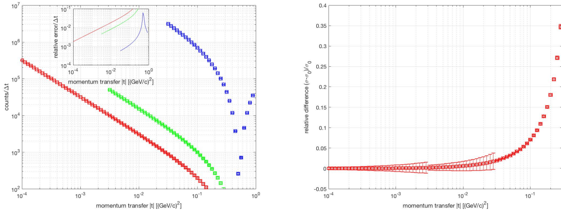
Figure 31: Left: Differential count rate dN/dt for elastic scattering events. The inset shows the relative statistical uncertainties expected. Right: Ratio of two possible scenarios with for \sqrt{\langle r_e^2 \rangle} = 0.84 fm and \sqrt{\langle r_e^2 \rangle} = 0.88 fm (the latter is denoted as \sigma_0 ). We assume a triple measurement with three targets.
