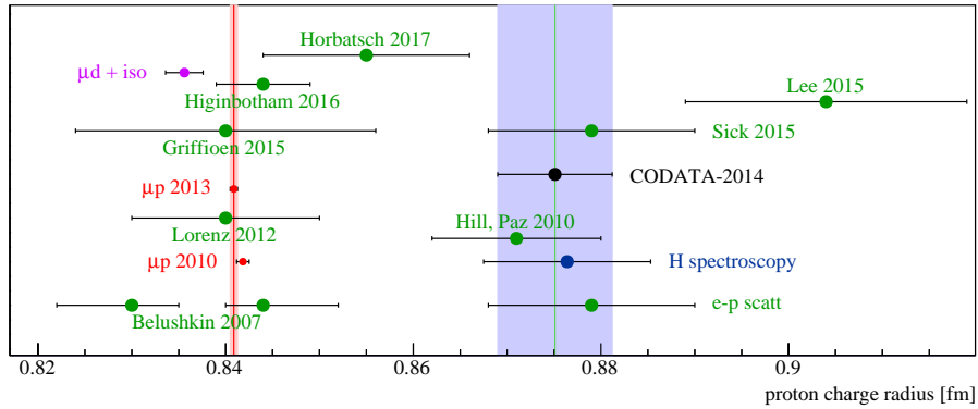
Figure 11: Proton radius from muonic hydrogen (red), hydrogen spectroscopy (blue) and electron-proton scattering (green). The CODATA value does not account for the muonic results. Figure is take from [47].
