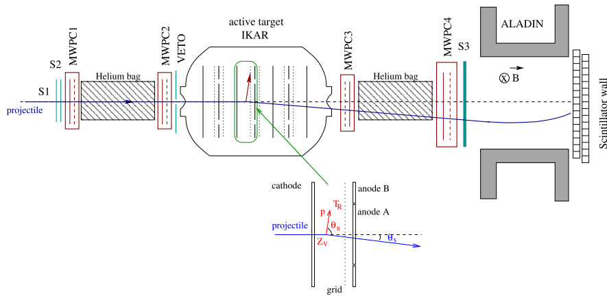
Figure 20: Example for the use of a high pressure active target TPC [56]
