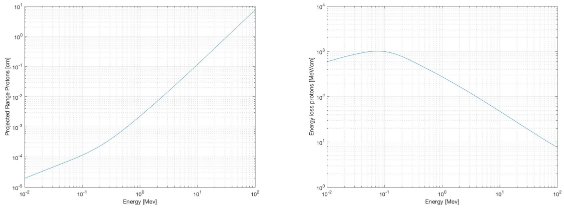
Figure 28: Projected range (left) and specific energy loss (right) for protons in scintillator for different kinetic energies [58].
