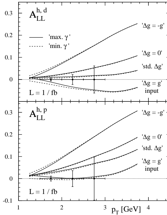
Figure 6.9: Double-spin asymmetry A_{LL}^{b,d} —single-inclusive production of charged hadrons ( p , \pi^\pm , K^\pm )—at next-to-leading order for different gluon polarizations in the nucleon, and minimal and maximal saturation of the polarized photon densities, dashed and solid lines, respectively (see text). The error bars indicate the estimated statistical uncertainty obtained with a luminosity of \mathcal{L} = 1 \text{ fb}^{-1} with COMPASS kinematics. Taken from [48].
