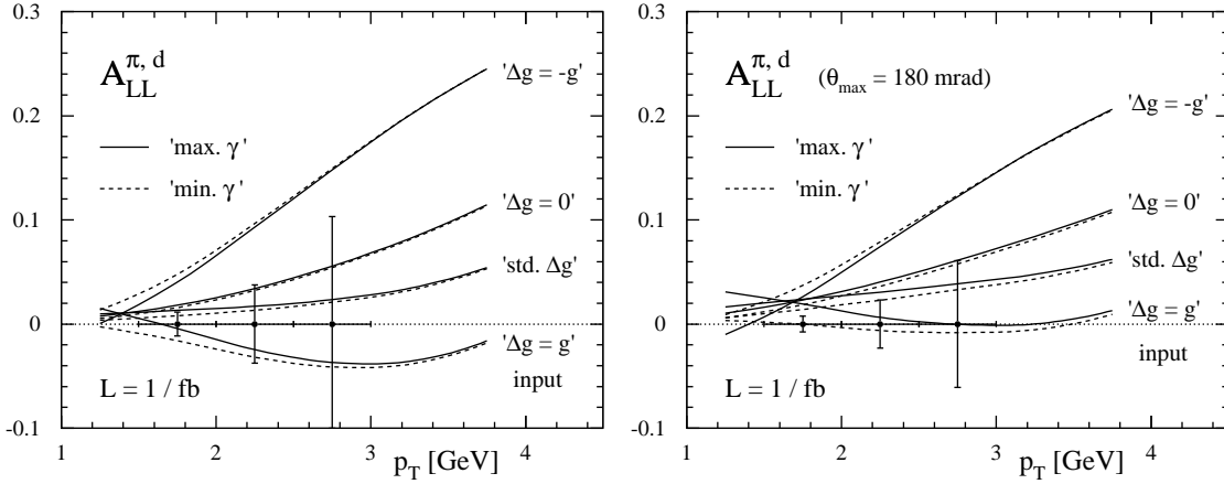
Figure 6.8: Double-spin asymmetry A_{LL}^{\pi, d} at next-to-leading order for different gluon polarizations in the nucleon and minimal and maximal saturation of the polarized photon densities (see text). The error bars indicate the estimated statistical uncertainty for \mathcal{L} = 1 \text{ fb}^{-1} with COMPASS kinematics. The right plot assumes the new COMPASS target magnet, which has not been used for the data taking periods of 2002 to 2004. Taken from [48].
