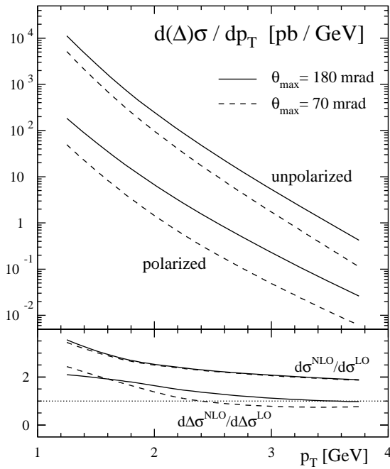
Figure 6.6: Unpolarized and polarized p_T -differential cross sections at next-to-leading order for the reaction \mu d \rightarrow \mu' \pi^0 X for SMC ( \theta_{\max} = 70 mrad) and COMPASS ( \theta_{\max} = 180 mrad) target magnets. The lower panel shows ratios of next-to-leading order to LO results ( K -factors). Taken from [48].
