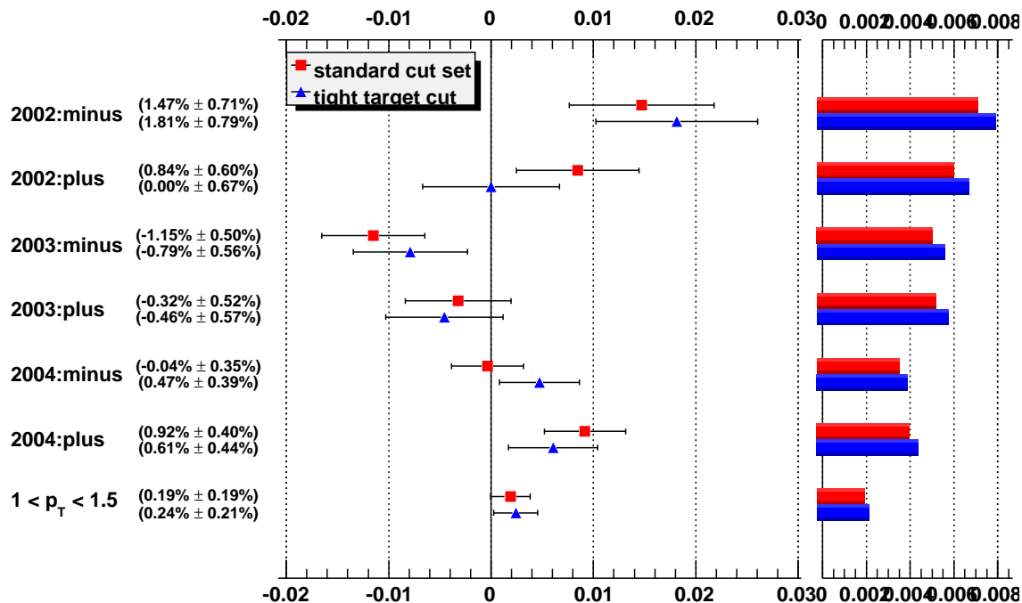
Figure 7.26: Study of different cut sets in the lowest p_T bin ( 1 \text{ GeV}/c < p_T < 1.5 \text{ GeV}/c ) split by beam time and microwave setting; the lowest points represent the weighted average of the asymmetries displayed above. For an in depth discussion see section 7.6.2. The pulls for the individual asymmetries pertaining to each data point are shown in figure D.13 on page 158.
