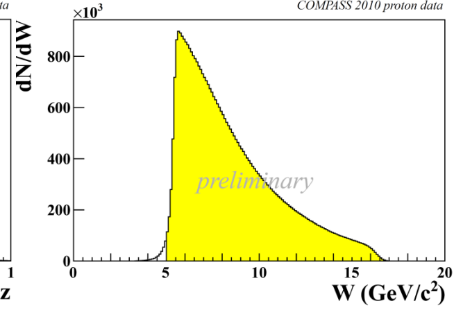
COMPASS 2010 proton data
