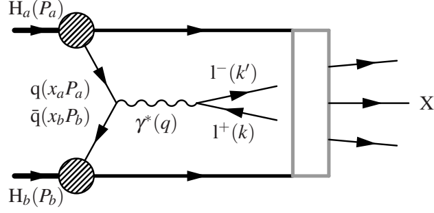
Figure 1: The Drell–Yan process. A quark-antiquark pair from the two hadrons annihilate, producing a lepton-antilepton pair in final state. The grey box denotes hadronization.
