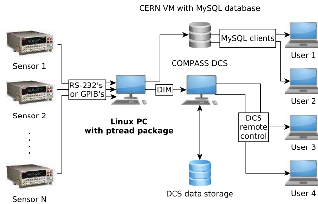
Figure 3: Diagram of pthread communication. The Linux computer with pthread package reads sensors. Data can be stored locally in SQLite database, sent to MySQL database and published by DIM server for COMPASS DCS.
