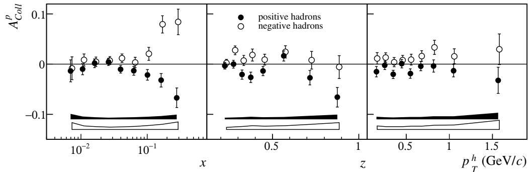
Figure 8. Collins asymmetry as a function of x , z , and p_T^h , for positive and negative hadrons. The bars show the statistical errors. Figure taken from [27].
