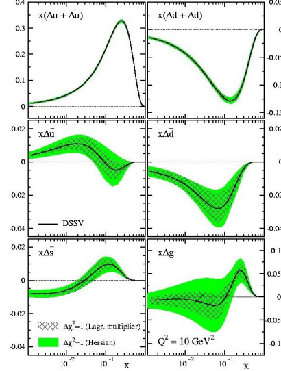
Figure 5. Results of the DSSV global parton analysis for the proton at Q^2 = 10 \text{ GeV}^2 , in the \overline{\text{MS}} scheme, [18].
