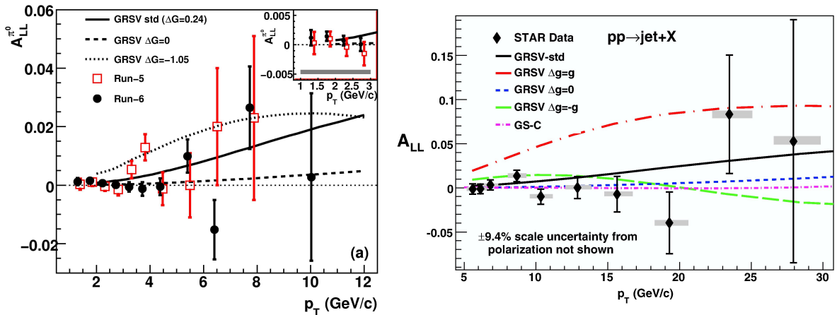
Figure 6. RHIC polarised proton–proton results at \sqrt{s} = 200 GeV. Curves mark different \Delta G scenarios. Left: PHENIX results, [19] for the asymmetry in \pi^0 production as a function of its p_T . Errors are statistical. Right: STAR results, [20] for the longitudinal double-spin asymmetry A_{LL} for inclusive jet production as a function of jet p_T . Errors are statistical.
