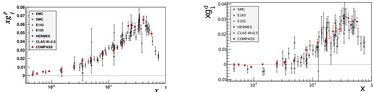
Figure 1. Results on xg_1^p (left) and xg_1^d (right) as a function of x for Q^2 > 1 \text{ GeV}^2 . Error bars represent the systematic and statistical uncertainties added in quadrature. The data have been evolved to Q^2 = 3 \text{ GeV}^2 .
