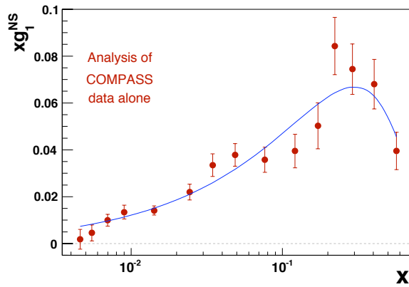
Figure 2: Preliminary values of g_1^{NS}(x) at Q^2 = 3(\text{GeV}/c)^2 . The curve represents the NLO QCD fit to the COMPASS data.
