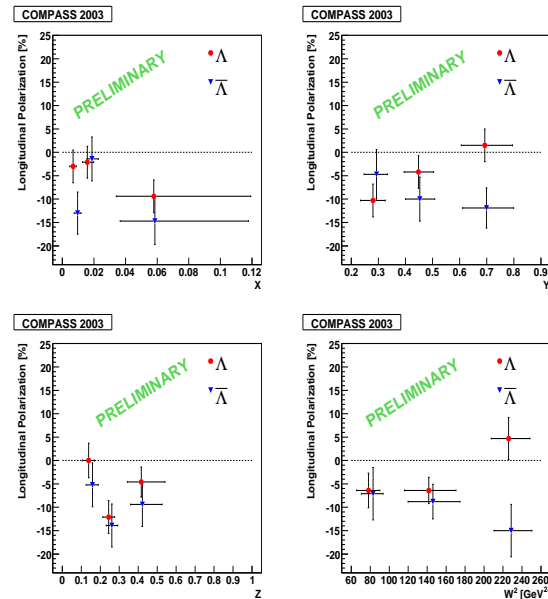
Figure 1. Dependence of the longitudinal \Lambda and \bar{\Lambda} polarization on x_{Bj} , y , z_\Lambda , and W^2 .
